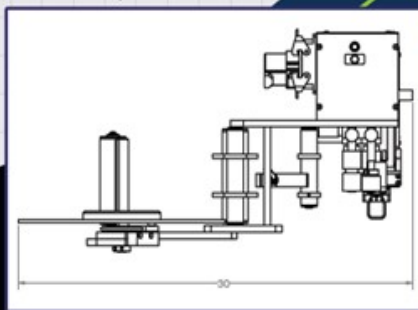
Dimensions, Head
